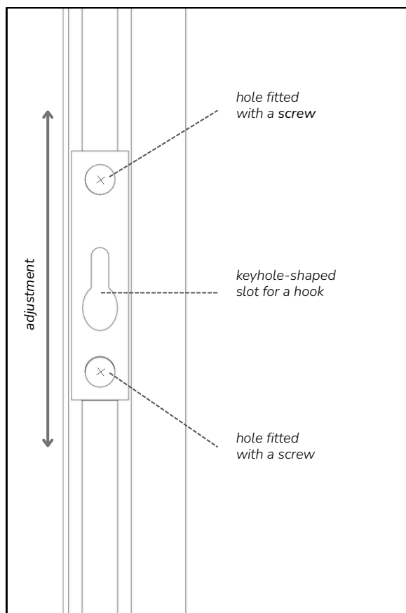
A close-up of the hanger showing the keyhole- shaped slot and two holes fitted with screws used to attach the hanger plate to the frame
